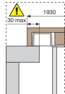
Particolare vasca ad incasso Particular of shell for built-in installation
